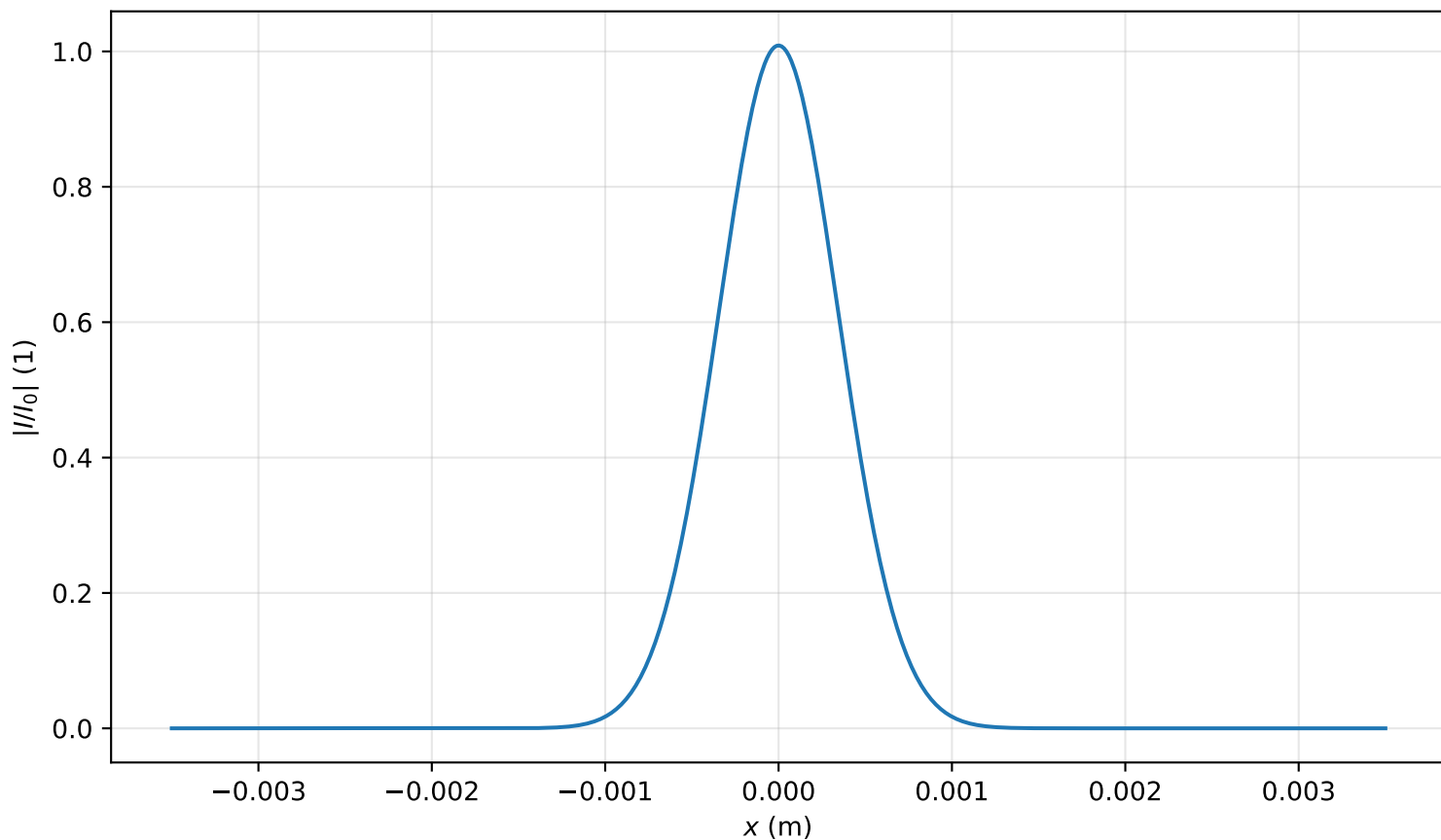
Intensity profile I(x, y = 0, z = 0.159m)/I_0 , P_{in}=0.6P_{cr} , artificial time
